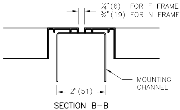
BOTH DIMENSIONS OVER 48" (1219) UP TO 144"x96" (3658x2438) MULLIONS AND MOUNTING CHANNEL
