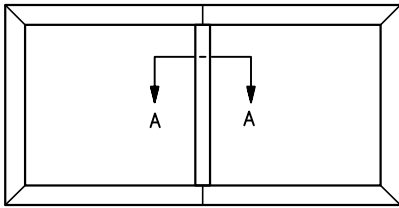
ONE DIMENSION OVER 48" (1219) SIZES UP TO 96"x48" (2438x1219) TWO SECTIONS WITH MULLION
